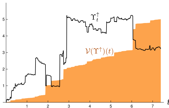
FIGURE 3. Simulation of the processes \gamma and V(\gamma) .
