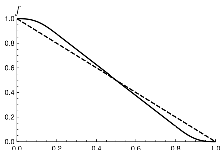
FIGURE 5. The solid curve corresponds to a function f satisfying the hypotheses of Lemma 6 with \alpha = 0.2 , while the dashed line depicts x \mapsto 1 - x .
