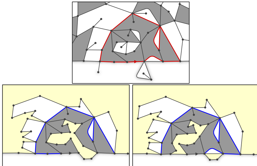
FIGURE 8. Illustration of the outer-most boundary of the percolation cluster: L = 12 is the number of edges on the red cycle and N = 9 and N^\theta = 9 are the number of edges on the blue path on the left and on the right respectively.
