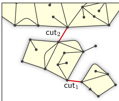
FIGURE 6. Illustration of the decomposition of M^{(\gamma)} .
