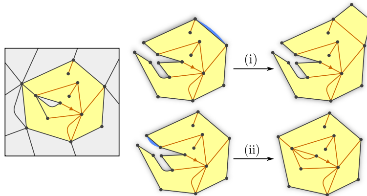
FIGURE 2. Illustration of a (filled-in) peeling step in a one-ended bipartite map. The peel edge is depicted in blue. In the first case we add a new face adjacent to this edge, and in the second case we identify two edges on the boundary of the hole (this identification can be made either to the left or to the right of the peel edge, so there are actually three cases); in the case (ii), the hole is split into two components and we fill-in the finite one.
