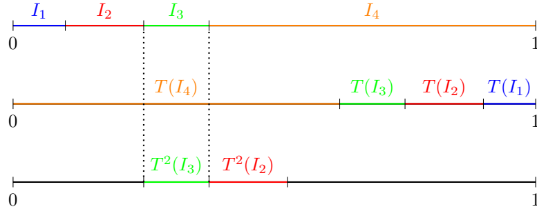
FIGURE 1. Plot of the exchanged intervals (and some of their iterates) for the symmetric IET T described in Example 3.15. The set \{\partial I_2, T(\partial I_2), T^2(\partial I_2) = \partial I_4\} defines a connection disjoint from the set \{c_\alpha \mid \alpha \in \mathcal{A} \cup 1/2\} . By Corollary 3.14, T is not ergodic.
