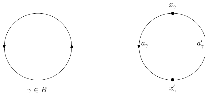
FIGURE 2.1. A closed orbit and integral curves
