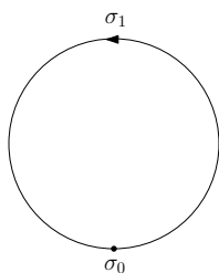
FIGURE 1.1. A triangulation on S^1 .
