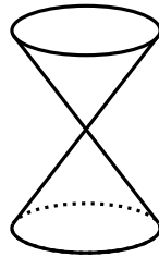
FIGURE 13. A cone singularity
