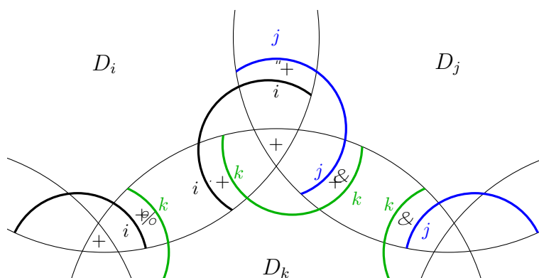
FIGURE 18. As we go clockwise around a positive vertex (center) the canonical section moves positively around the fiber circle i \rightarrow j \rightarrow k \rightarrow i giving winding number -1 . As we go counterclockwise around the midpoint of the edge E_{ik} connecting two positive vertices, we go from i to k back to i in the positive direction giving winding number +1 . Around the midpoint of an E_{jk} connecting positive and negative vertices we go positively from j to k then negatively from k to j giving winding number zero.
