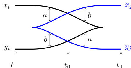
FIGURE 21. Portion of the front projection of \Lambda_G lying over a curve transverse to an edge of G : t, t_0, t_+ are parameter values along this curve. The critical points y_i, y_j have index 2k and x_i, x_j have index 2k + 1 . The four two-headed vertical arrows indicate the possible handle slides which we claim must be: y_{ij}^b, x_{ji}^a, x_{ij}^b, y_{ji}^a .
