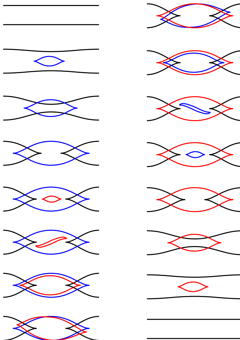
FIGURE 6. The mesh Legendrian \Lambda_G corresponding to the G of Figure 5 consists of three components, one black, one blue and one red. Its front \pi(\Lambda_G) is a subset of J^0(S^2) = S^2 \times \mathbb{R}_z . We think of S^2 as \mathbb{R}_{x,y}^2 compactified at infinity and draw \pi(\Lambda_G) as a movie of 1-dimensional fronts \Sigma_y \subset J^0(\mathbb{R}_x) = \mathbb{R}_x \times \mathbb{R}_z , fixed at infinity, where y is the time coordinate. We will see that \Lambda_G is generated by a function f : S^3 \rightarrow \mathbb{R} , where we view S^3 as the total space of the Hopf fibration S^1 \rightarrow S^3 \rightarrow S^2 . The Legendrian \Lambda_G is a Borromean link in the sense that any two of the three components of \Lambda_G form a trivial Legendrian link, but the three together form a nontrivial Legendrian link. Moreover, \Lambda_G is trivial as a formal Legendrian link.
