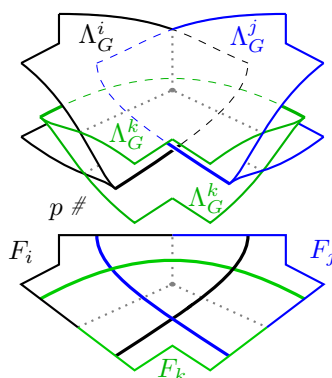
FIGURE 4. Components \Lambda_G^i , \Lambda_G^j , \Lambda_G^k spiral positively around a positive vertex in G . The i th cusp line (black) goes under the j th cusp line (blue).
