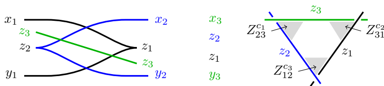
FIGURE 22. Critical points of the lower index 2k are denoted y_i . The upper index critical points are x_i . Corresponding birth-death points are indicated by z_i . The triangle on the right is the triangle of birth death lines projected to the base with overcrossing indicating that z_3 is above z_2 , etc. at the corners. The shaded region indicates the position of possible exchange points. The critical values of x_3, y_3, z_1, z_2 at the bottom corner are indicated by the figure in the middle. On the left side is a possible graphic for the function along the z_3 birth-death line with possible exchanges indicated with \cdot . See also Figure 4 and the left side of 25 showing the same thing.
