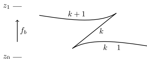
FIGURE 10. If the zig-zag is disjoint from the rest of the front, H(f_b^{-1}[z_0, z_1], f_b^{-1}(z_0)) would be the same at both endpoints. But this relative homology in degree k - 1 is zero on the left end and nonzero on the right end.
