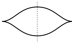
FIGURE 26. An “eye” (homeomorphic to S^1 ) in \mathbb{R}^2 = J^0(\mathbb{R}) . Spin this around the dotted line to get a “lens” (homeomorphic to S^2 ) in \mathbb{R}^3 = J^0(\mathbb{R}^2) .
