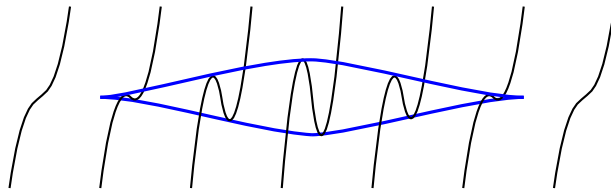
FIGURE 8. A 1-parameter family of functions generating an “eye” shaped Cerf diagram.
