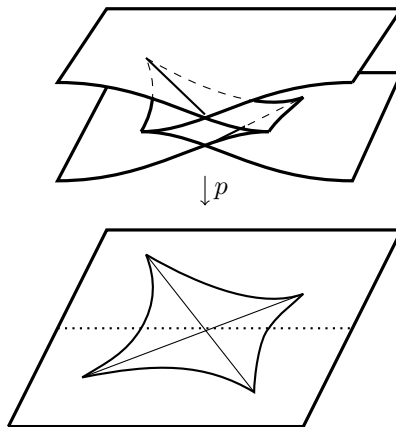
FIGURE 14. The Legendrian of Dimitroglou-Rizell cut over dotted line to show details.
