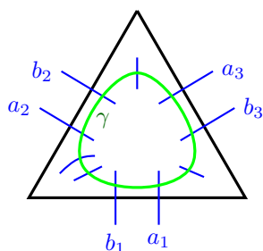
FIGURE 23. The curve \gamma .
