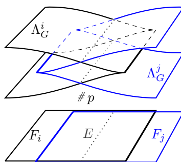
FIGURE 3. Two components \Lambda_G^i, \Lambda_G^j are linked over the edge E .
