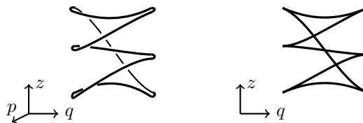
FIGURE 9. Legendrian submanifold of J^1\mathbb{R} on left with front projection on right. This Legendrian cannot be generated by any family of functions.
