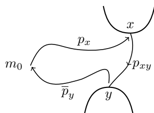
FIGURE 15. The paths p_x from m_0 to each critical point x are compatible with the Euler structure if each composition p_x \# p_{xy} \# \bar{p}_y is null homotopic.
