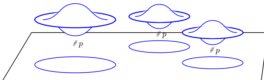
FIGURE 20. A disjoint union of flying saucers lying over disjoint balls.
