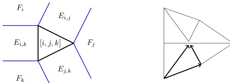
FIGURE 19. The cyclic poset on a positive triangle coming from a positive vertex in a ribbon graph is shown. For a negative triangle we reverse all the cyclic orders. As morphisms in the category of cyclic sets and inclusions, this gives six 2-simplices. Each gives a contribution of c_{\mathcal{Z}}(fkg, f_j, kg, f_i, j, kg) = 1/12 to the Euler number of the covering for a total of 1/2 for each positive vertex.
