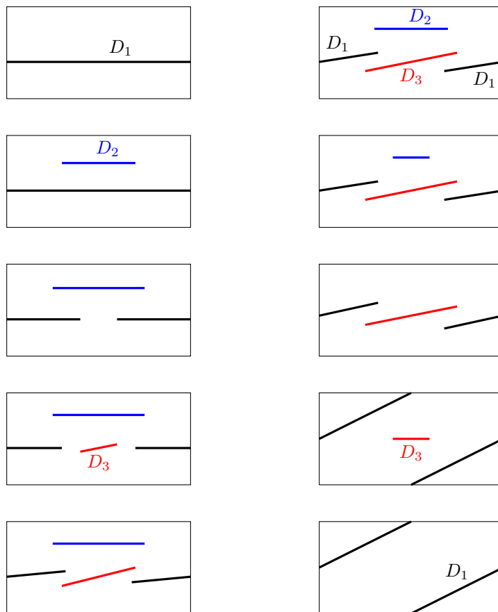
FIGURE 17. A system of 3 disks D_1, D_2, D_3 in E the Hopf circle bundle over S^2 is shown in this sequence of cross-sections of these disks. This gives the fiberwise PGMF illustrated in Figure 6.
