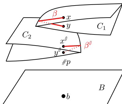
FIGURE 16. Given that C_1, C_2 are simply connected, a \rho -compatible weak Euler structure on F_b is given by choosing a path \alpha from x to y so that \gamma = \alpha \# \beta is in the kernel of \rho , where \beta is any path from x to y in C_1 and similarly for x^0, y^0 .
