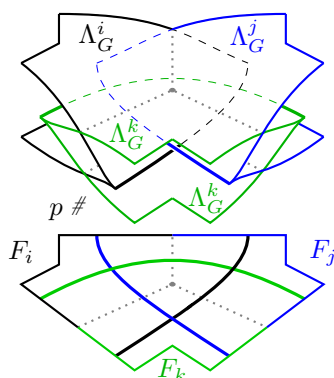
FIGURE 4. Components \Lambda_G^i , \Lambda_G^j , \Lambda_G^k spiral positively around a positive vertex in G . The i th cusp line (black) goes under the j th cusp line (blue).
