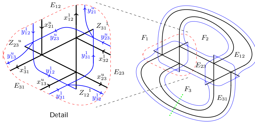
FIGURE 25. The black lines indicate k + 1/k + 1 handle slides x_{ij}^a giving column operations in the incidence matrices. The blue lines indicate k/k handle slides y_{ij}^b giving row operations. Exchange point, denoted Z_{ij}^c , is where the i th upper index critical point slides under the j th lower index critical point. The green dotted line indicates a discontinuity in the labeling. This is the “cut” that appears in the proof of Theorem 4.22. The triangles are two black vertices connected by three edges of the ribbon graph labeled E_{ij} .
