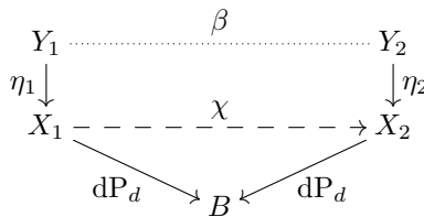
FIGURE 2. A Bertini link
