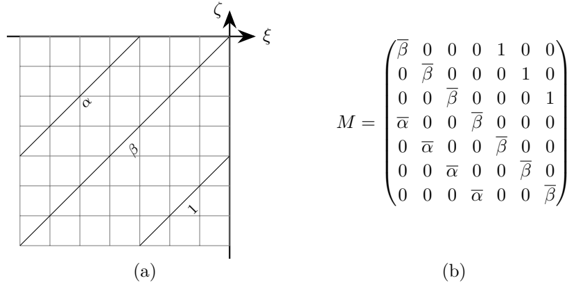
FIGURE 4.2. Construction of the matrix M from S^* in the case L = 3/7 .
